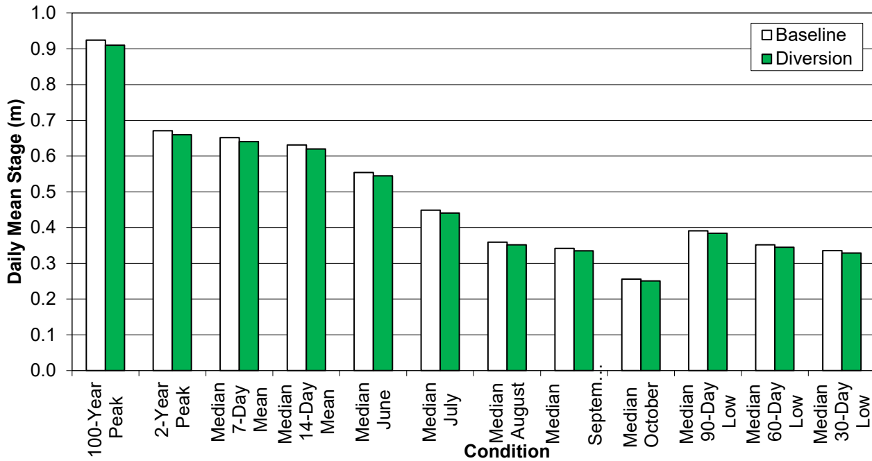
Figure 3: Derived Water Level Regimes at Meliadine Lake during the Baseline and Diversion Scenarios
