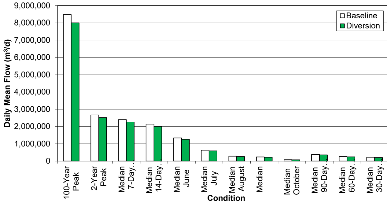
Figure 2: Derived Flow Regimes at Meliadine Lake during the Baseline and Diversion Scenarios
