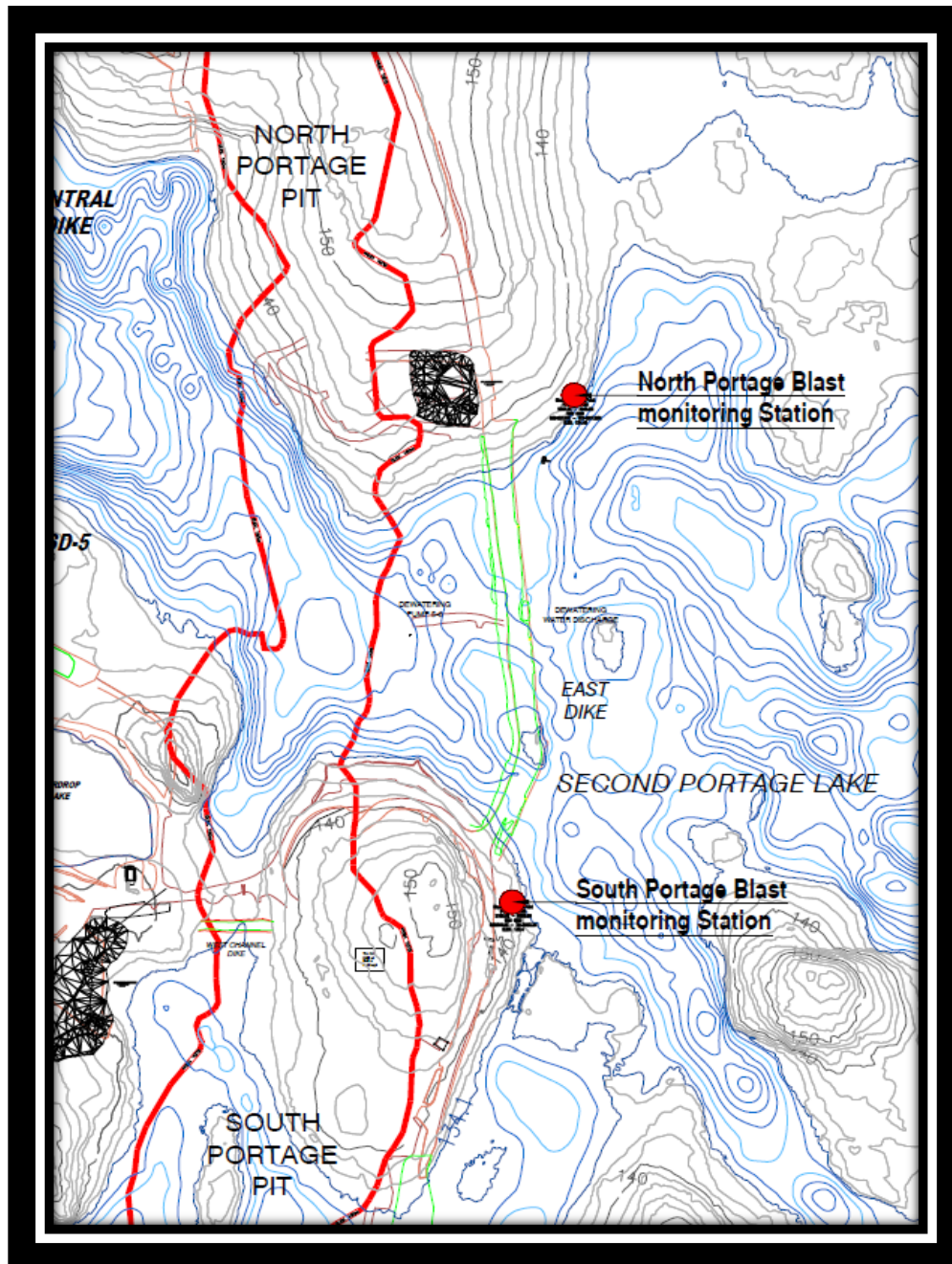
Figure 7: Localization of the two blast monitoring stations at Portage Pit
