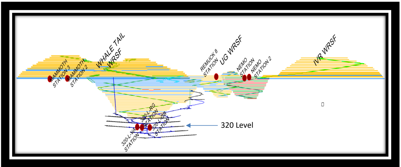
Figure 11: Localization of the blast monitoring stations at Whale Tail Site 320 Level
