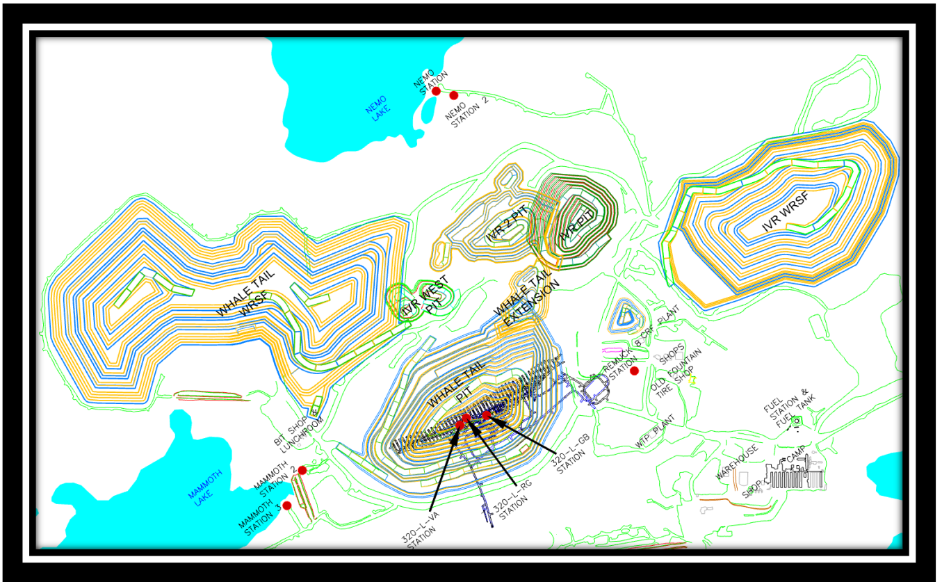
Figure 10: Localization of the blast monitoring stations at Whale Tail Site with Underground mine
