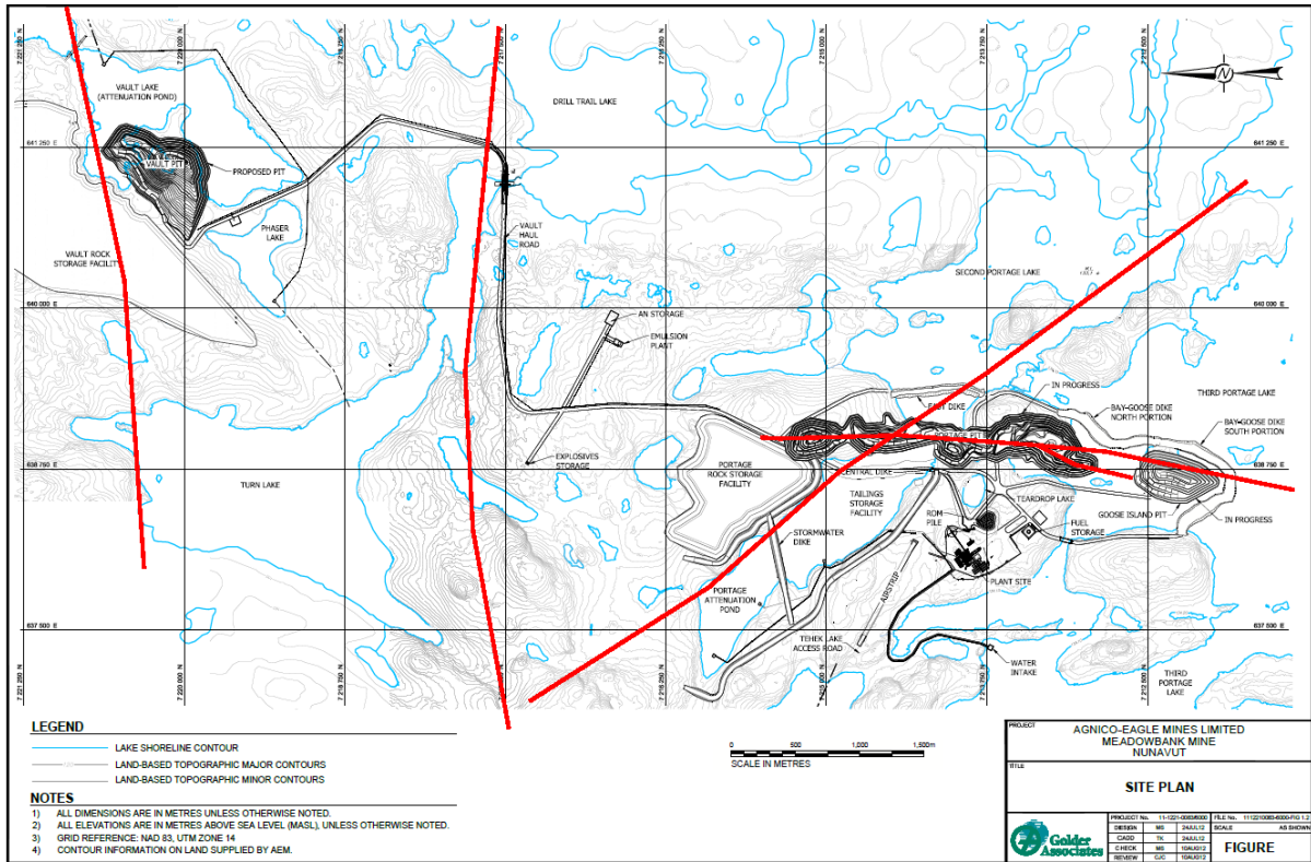
Figure 2-5: Inferred Locations of Faults
