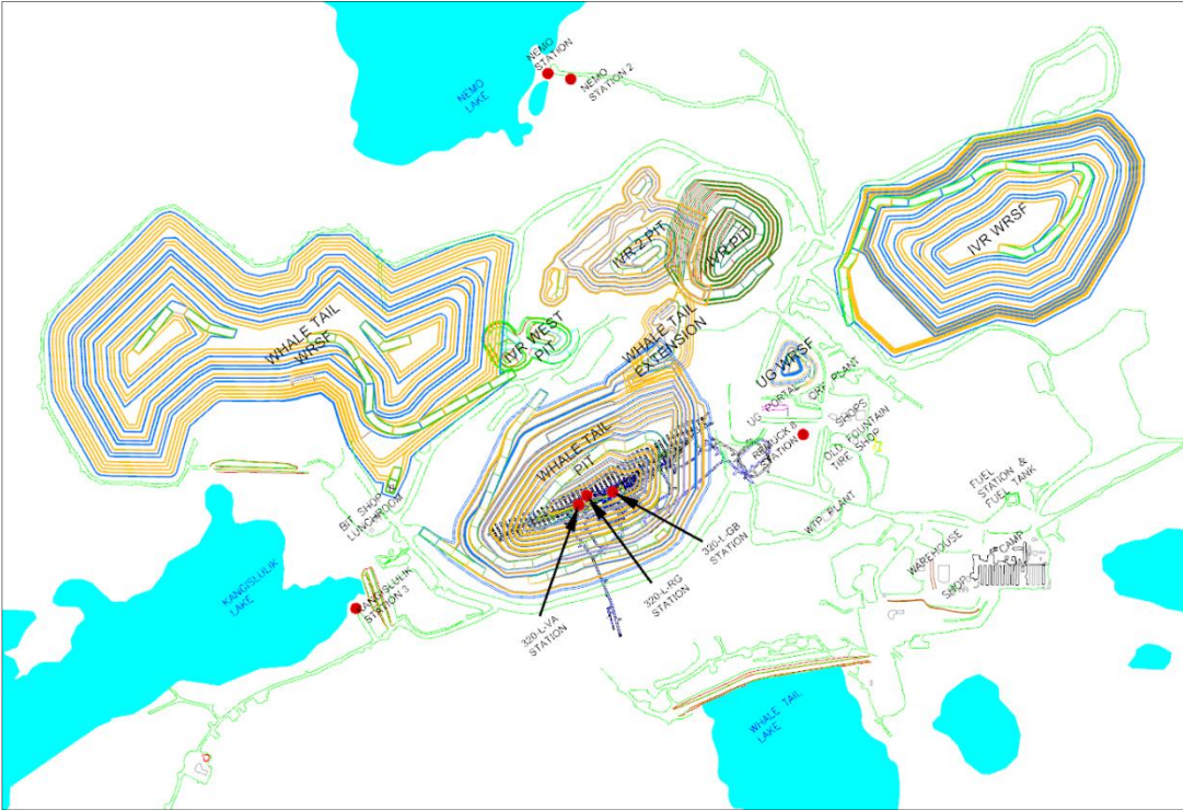
Figure 11: Localization of the blast monitoring stations at Whale Tail Site with UG mine
