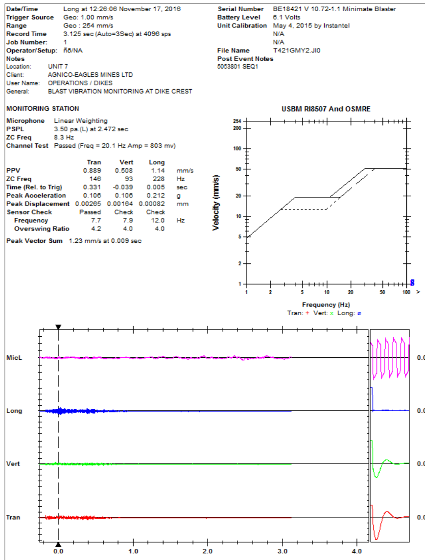
Figure 13: Example of the blast monitoring results
