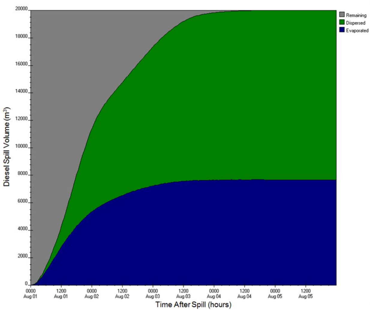
Figure E-A58: ADIOS2 diesel fuel budget output for Hudson Bay crossing station (5A) for 20,000 m 3 , mean wind speed scenario
