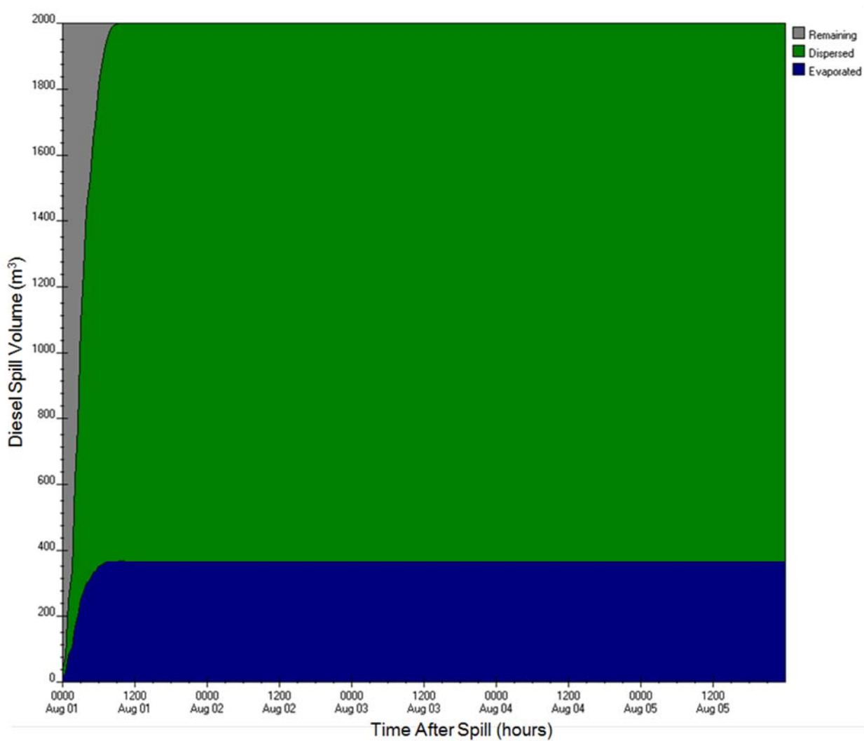
Figure E-A62: ADIOS2 diesel fuel budget output for Western Hudson Strait, Charles Island station (6A) for 2,000 m 3 , 2-yr wind speed scenario
