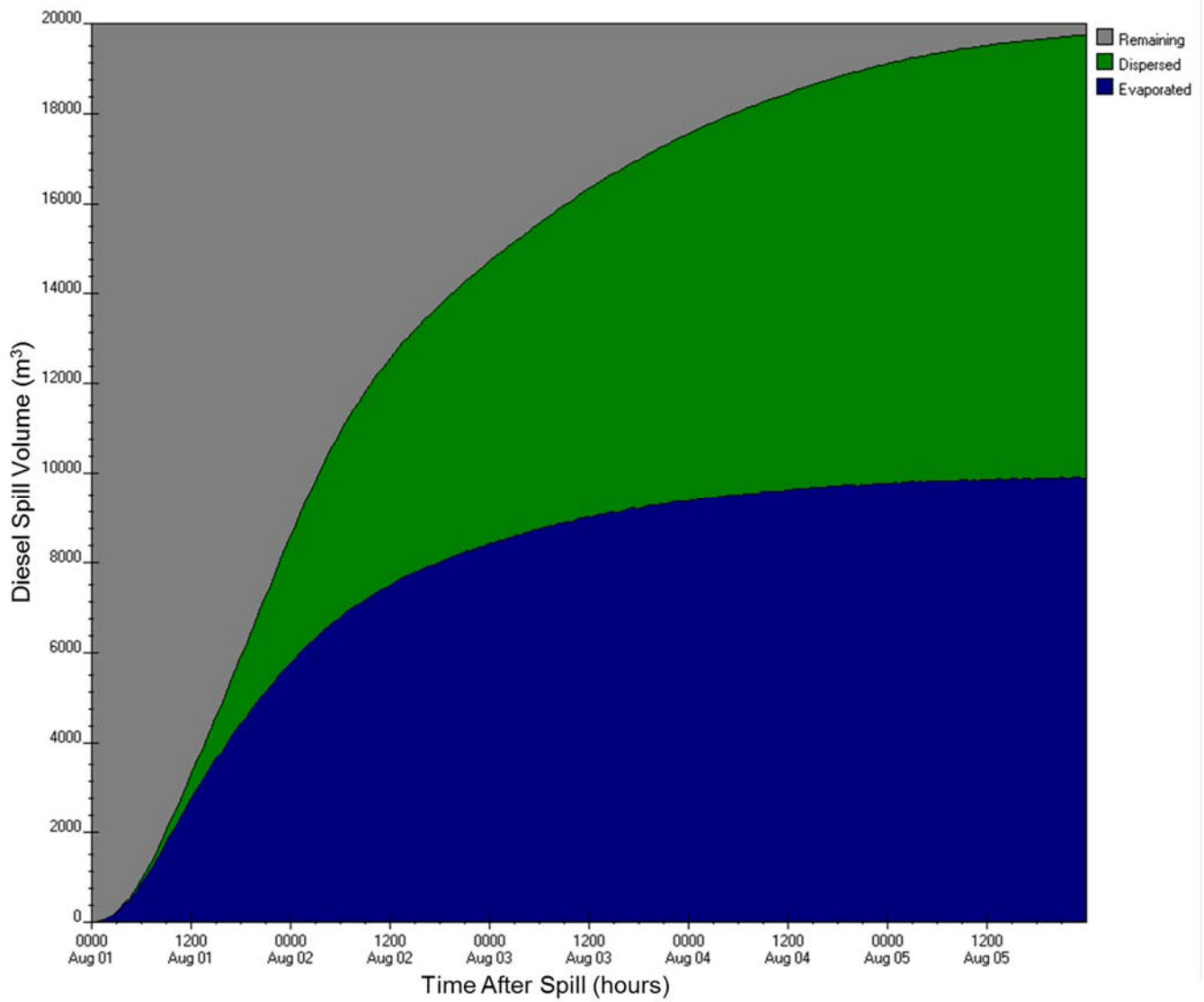
Figure E-A13: ADIOS2 diesel fuel budget output for Walrus Island station (3) for 20,000 m 3 , mean wind speed scenario
