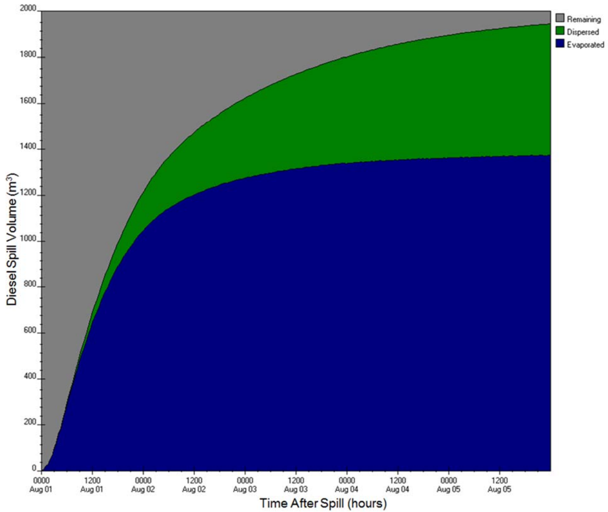
Figure E-A37: ADIOS2 diesel fuel budget output for West and East Melvin Bay stations (1A and 2A) for 2,000 m 3 , mean wind speed scenario
