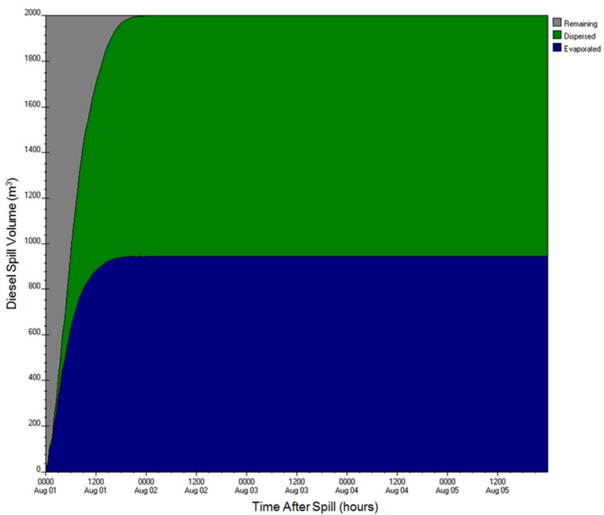
Figure E-A44: ADIOS2 diesel fuel budget output for Entrance to Melvin Bay station (3A) for 2,000 m 3 , 2-yr wind speed scenario
