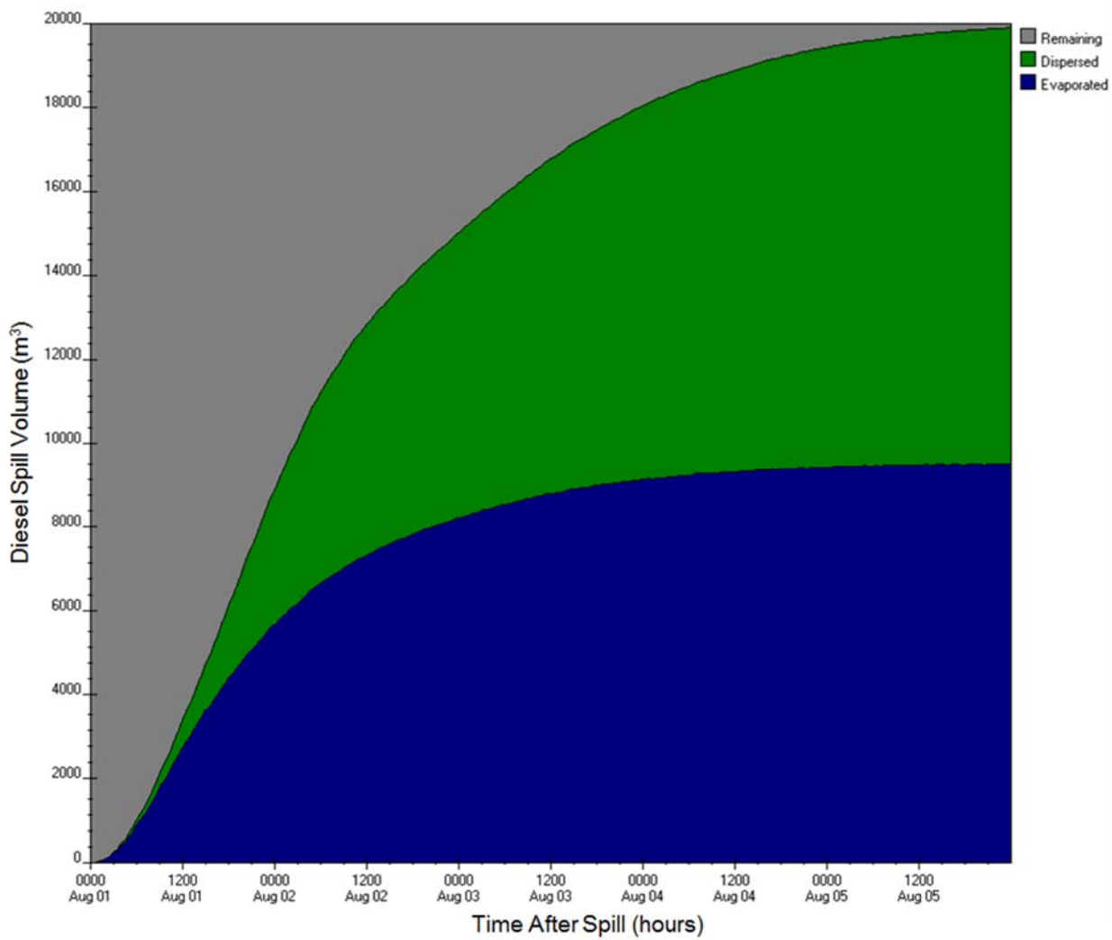
Figure E-A64: ADIOS2 diesel fuel budget output for Western Hudson Strait, Charles Island station (6A) for 20,000 m 3 , mean wind speed scenario
