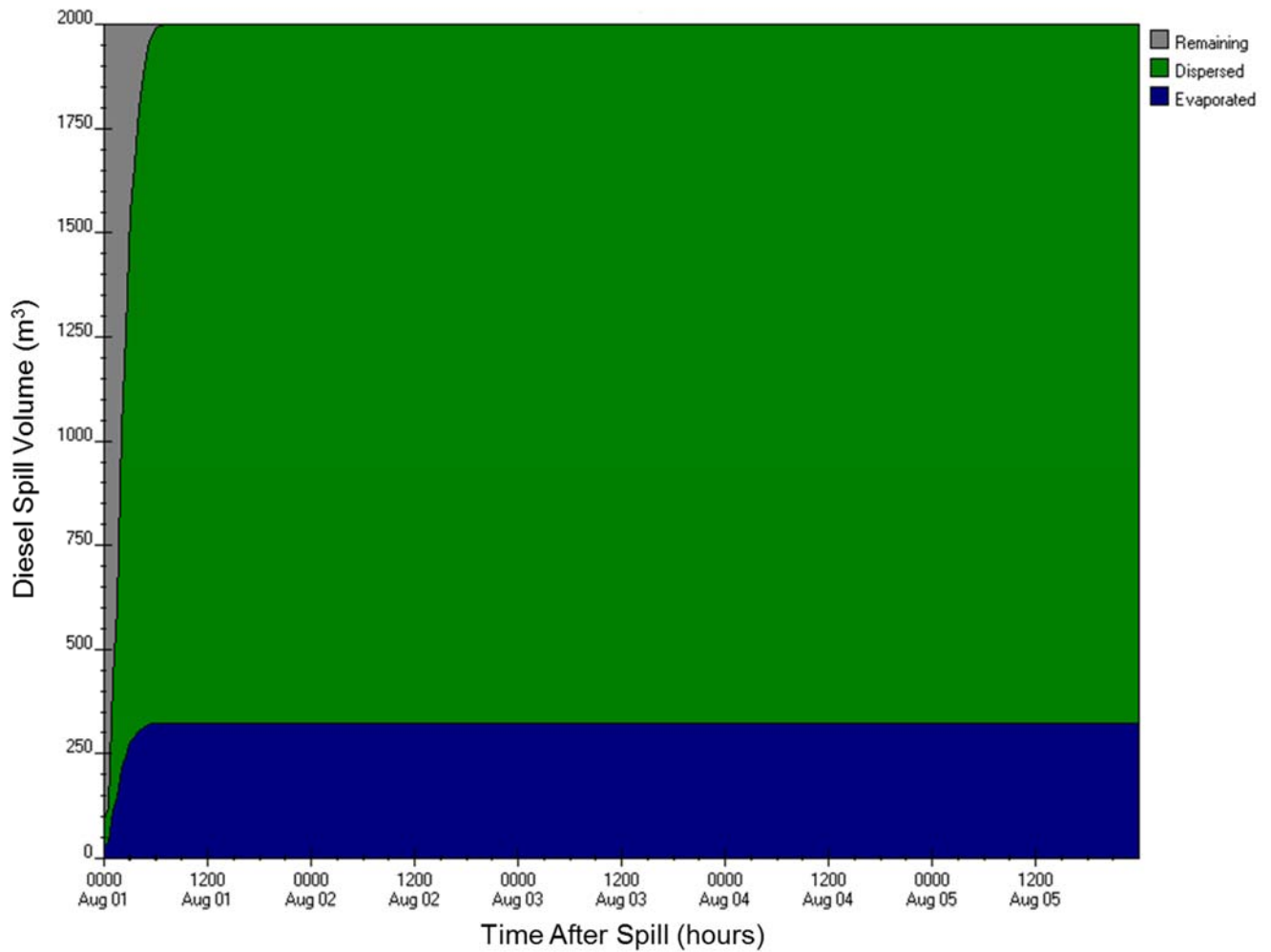
Figure E-A12: ADIOS2 diesel fuel budget output for Walrus Island station (3) for 2,000 m 3 , 50-yr wind speed scenario
