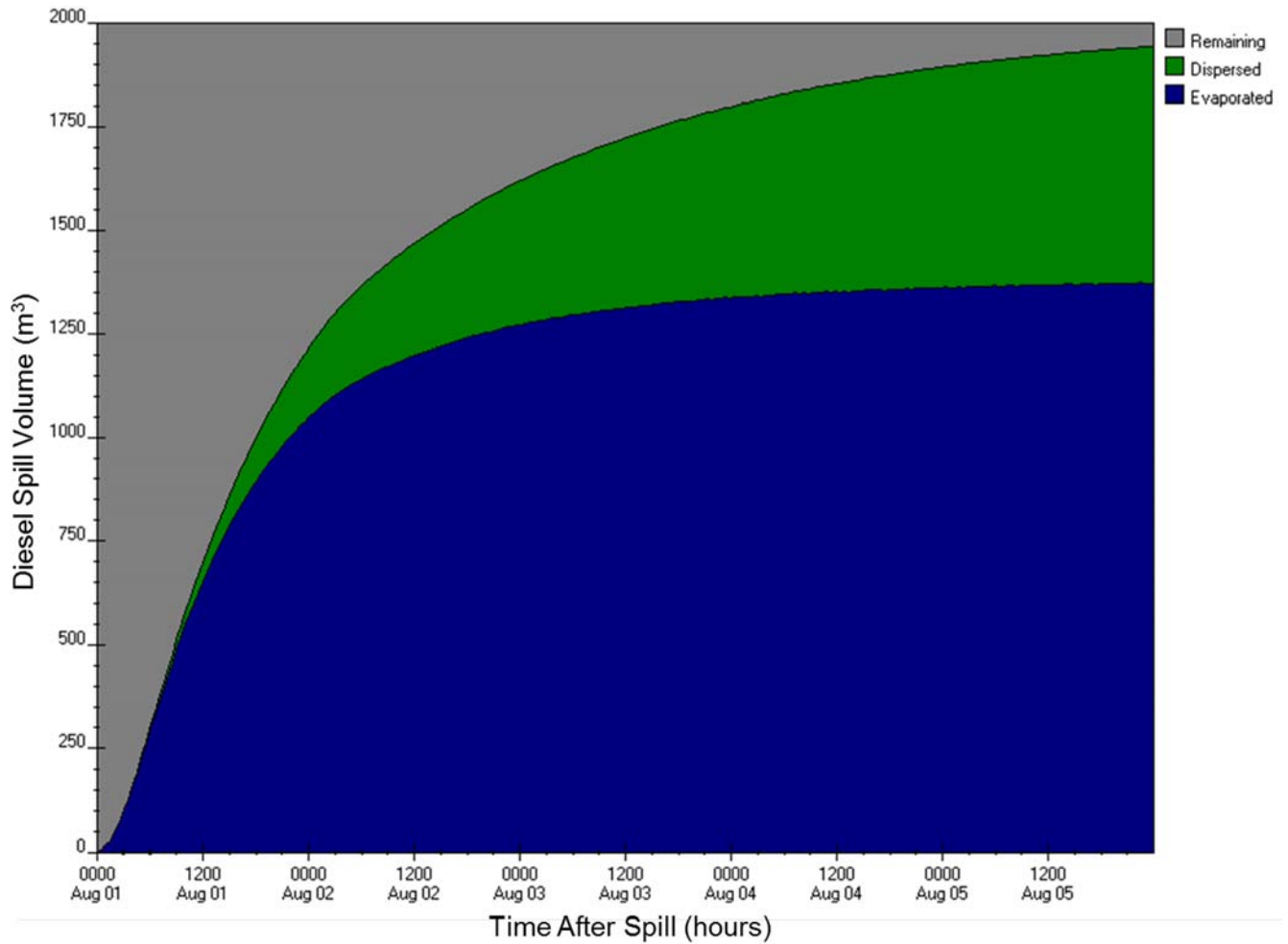
Figure E-A4: ADIOS2 diesel fuel budget output for two fuel transfer stations (1 and 2) near Melvin Bay for 2,000 m 3 spill, mean wind speed scenario
