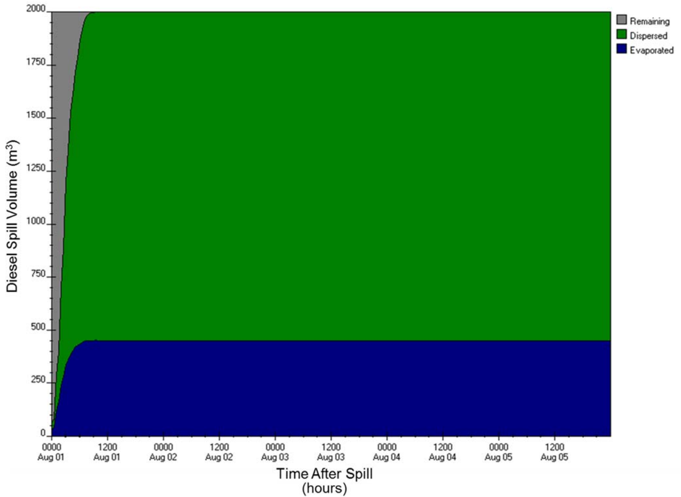
Figure E-A18: ADIOS2 diesel fuel budget output for Coats Island station (4) for 2,000 m 3 , 50-yr wind speed scenario
