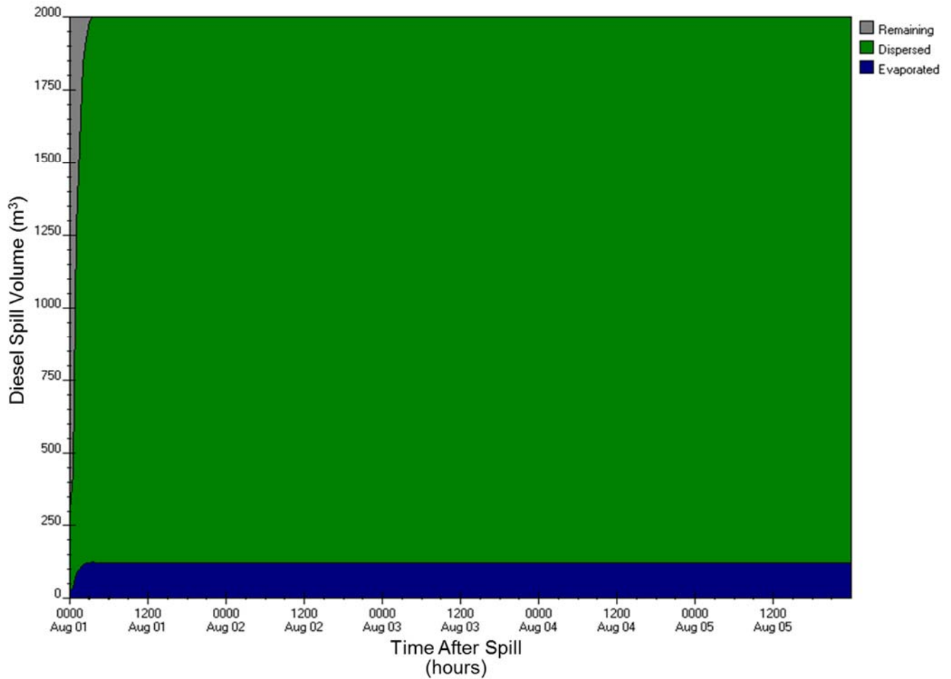
Figure E-A30: ADIOS2 diesel fuel budget output for Eastern Hudson Strait station (6) for 2,000 m 3 , 50-yr wind speed scenario
