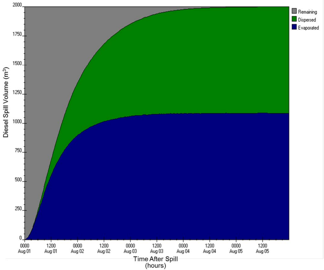
Figure E-A28: ADIOS2 diesel fuel budget output for Eastern Hudson Strait station (6) for 2,000 m 3 , mean wind speed scenario
