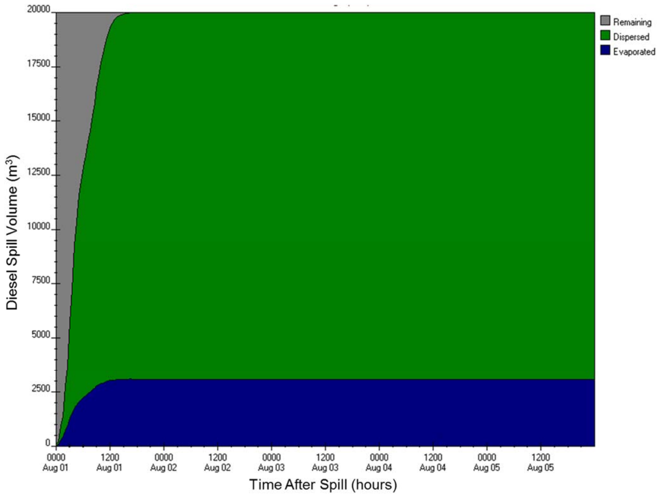
Figure E-A-15: ADIOS2 diesel fuel budget output for Walrus Island station (3) for 20,000 m 3 , 50-yr wind speed scenario
