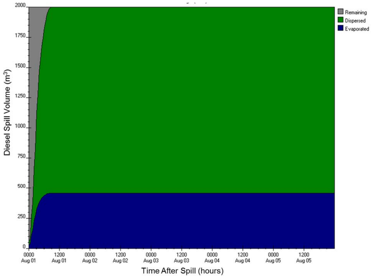
Figure E-A74: ADIOS2 diesel fuel budget output for Eastern Hudson Strait station (8A) for 2,000 m 3 , 50-yr wind speed scenario
