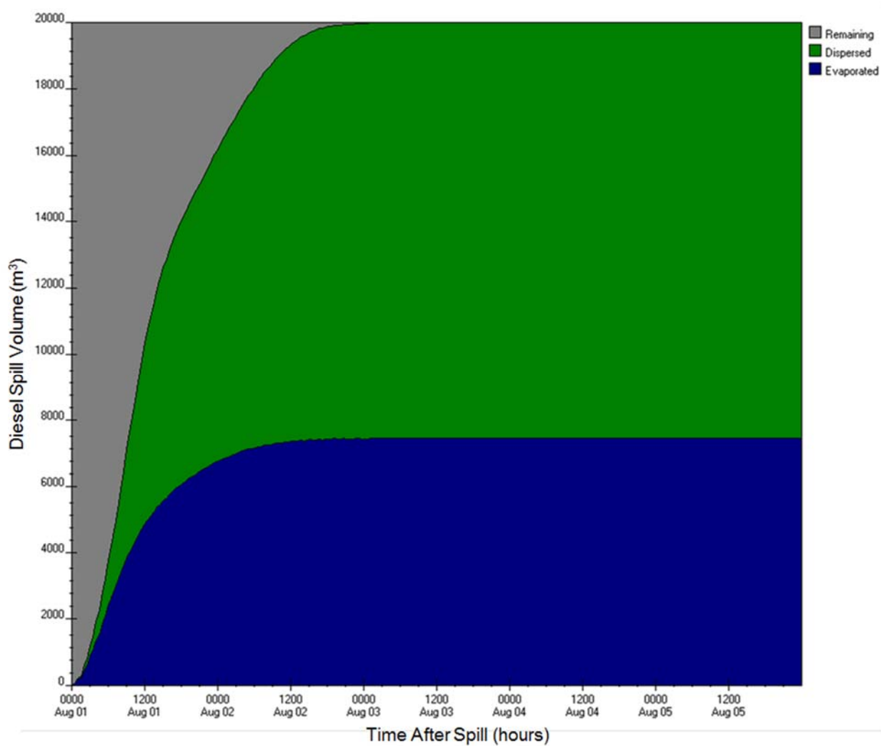
Figure E-A53: ADIOS2 diesel fuel budget output for West Hudson Bay station (4A) for 20,000 m 3 , 2-yr wind speed scenario
