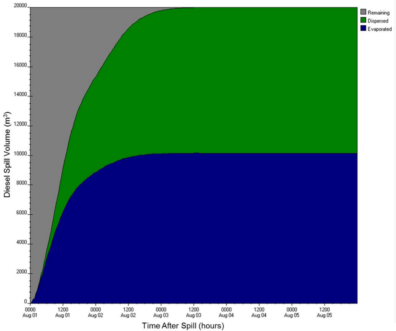
Figure E-A9: ADIOS2 diesel fuel budget output for two fuel transfer stations (1 and 2) near Melvin Bay for 20,000 m 3 , 50-yr wind speed scenario
