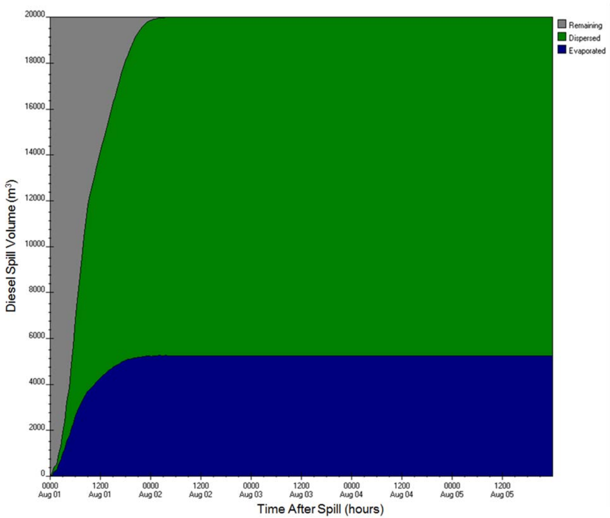
Figure 8.2-B-B-76: ADIOS2 diesel fuel budget output for Eastern Hudson Strait station (8A) for 20,000 m 3 , 2-yr wind speed scenario
