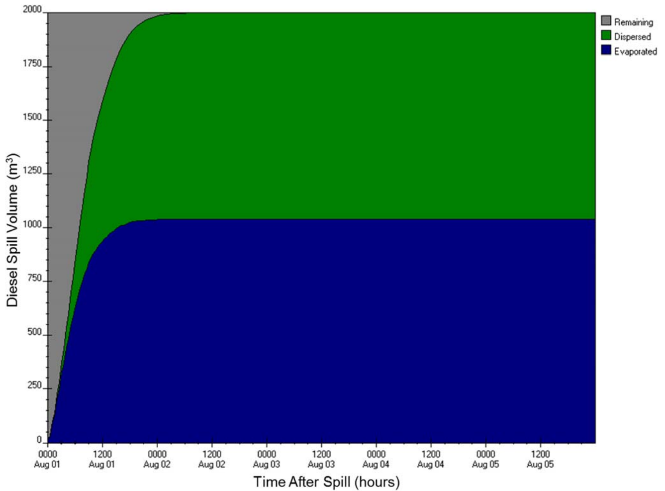
Figure E-A6: ADIOS2 diesel fuel budget output for two fuel transfer stations (1 and 2) near Melvin Bay for 2,000 m 3 , 50-yr wind speed scenario
