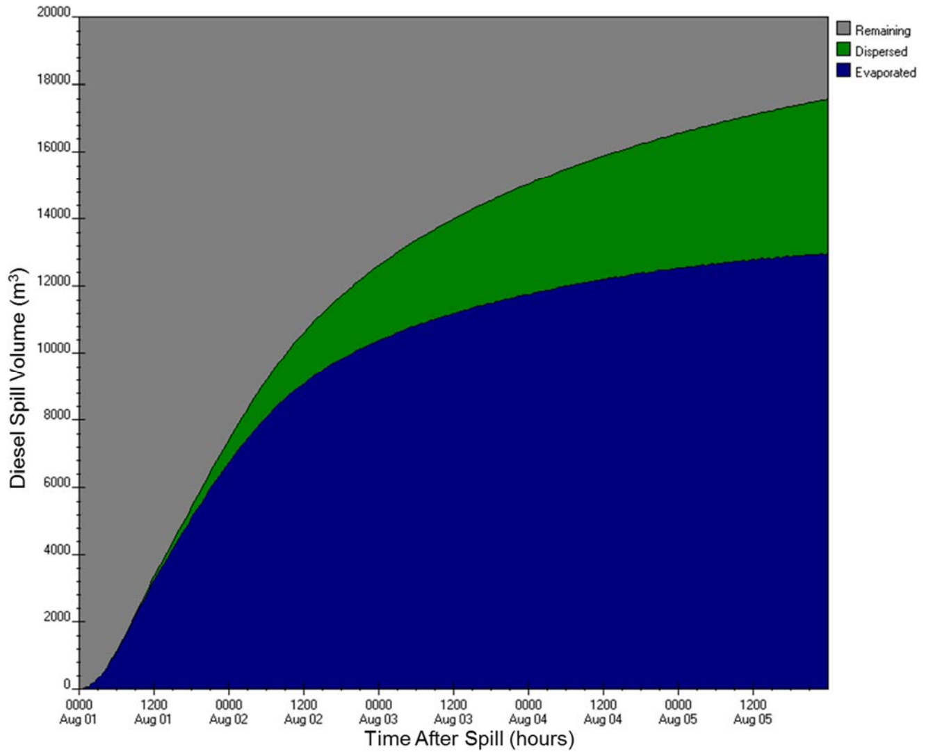
Figure E-A7: ADIOS2 diesel fuel budget output for two fuel transfer stations (1 and 2) near Melvin Bay for 20,000 m 3 spill, mean wind speed scenario
