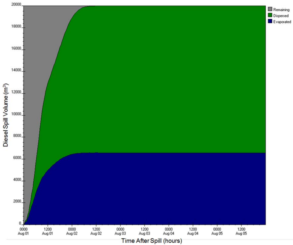
Figure E-A54: ADIOS2 diesel fuel budget output for West Hudson Bay station (4A) for 20,000 m 3 , 50-yr wind speed scenario
