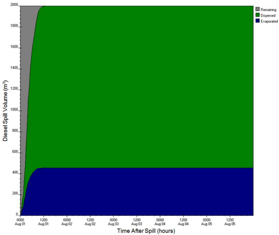
Figure E-A56: ADIOS2 diesel fuel budget output for Hudson Bay crossing station (5A) for 2,000 m 3 , 2-yr wind speed scenario
