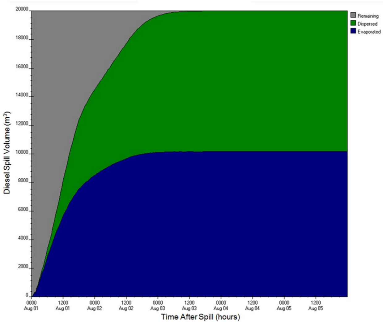
Figure E-A42: ADIOS2 diesel fuel budget output for West and East Melvin Bay stations (1A and 2A) for 20,000 m 3 , 50-yr wind speed scenario
