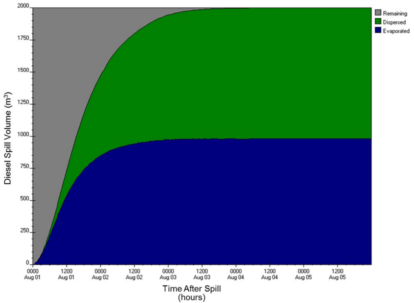
Figure E-A16: ADIOS2 diesel fuel budget output for Coats Island station (4) for 2,000 m 3 , mean wind speed scenario
