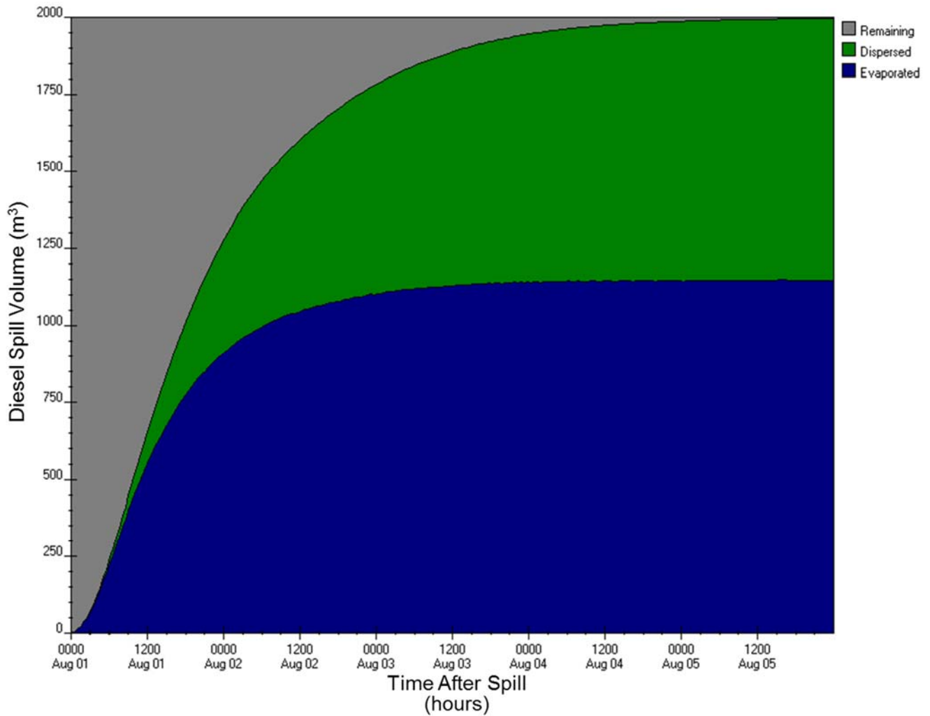
Figure E-A22:ADIOS2 diesel fuel budget output for Ungava Peninsula station (5) for 2,000 m 3 , mean wind speed scenario
