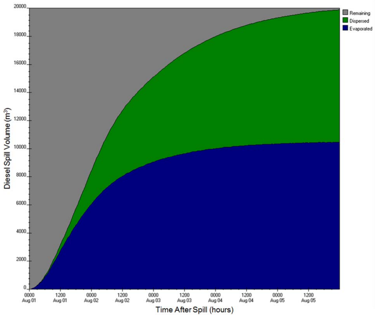
Figure E-A52: ADIOS2 diesel fuel budget output for West Hudson Bay station (4A) for 20,000 m 3 , mean wind speed scenario
