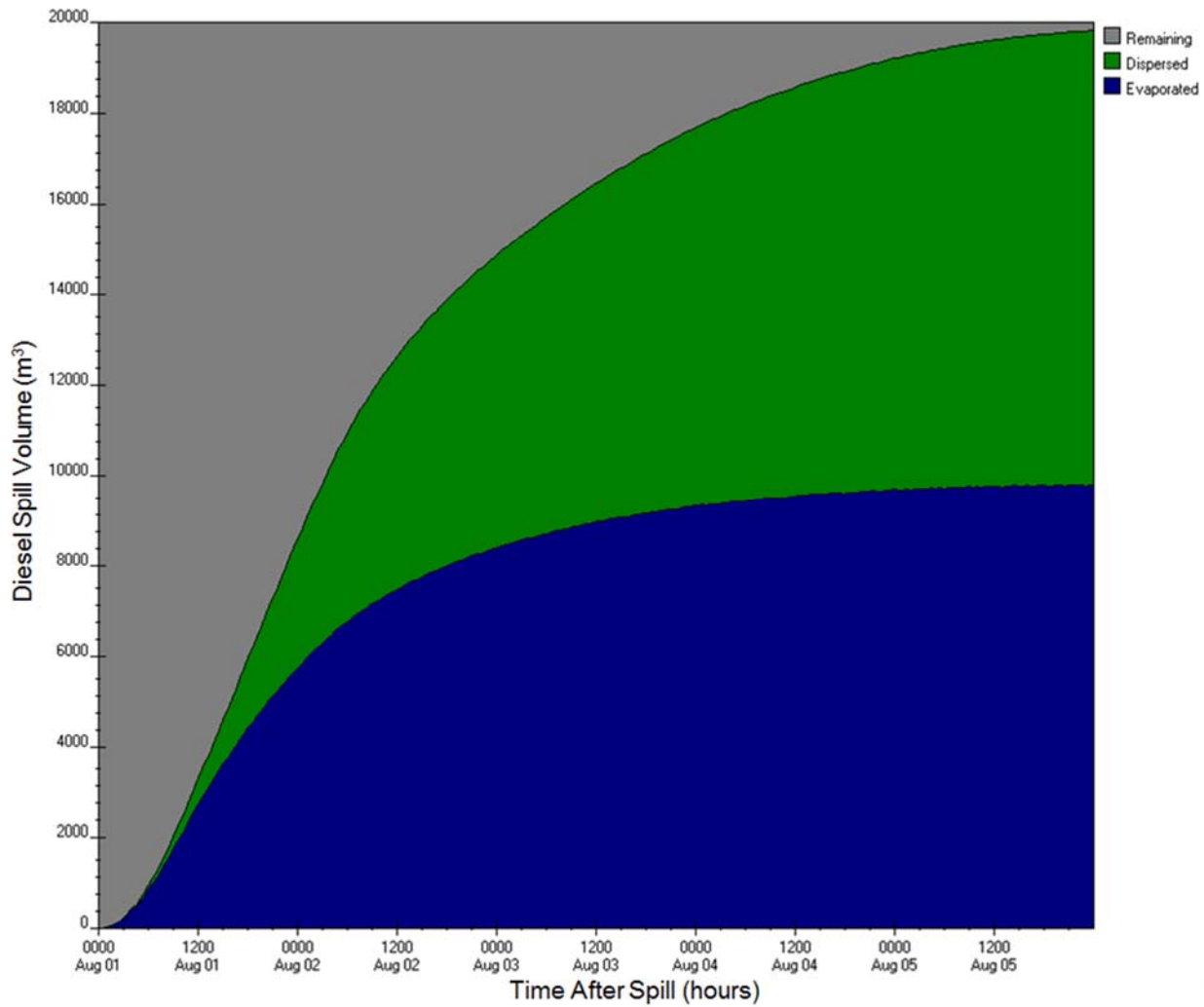
Figure E-A75: ADIOS2 diesel fuel budget output for Eastern Hudson Strait station (8A) for 20,000 m 3 , mean wind speed scenario
