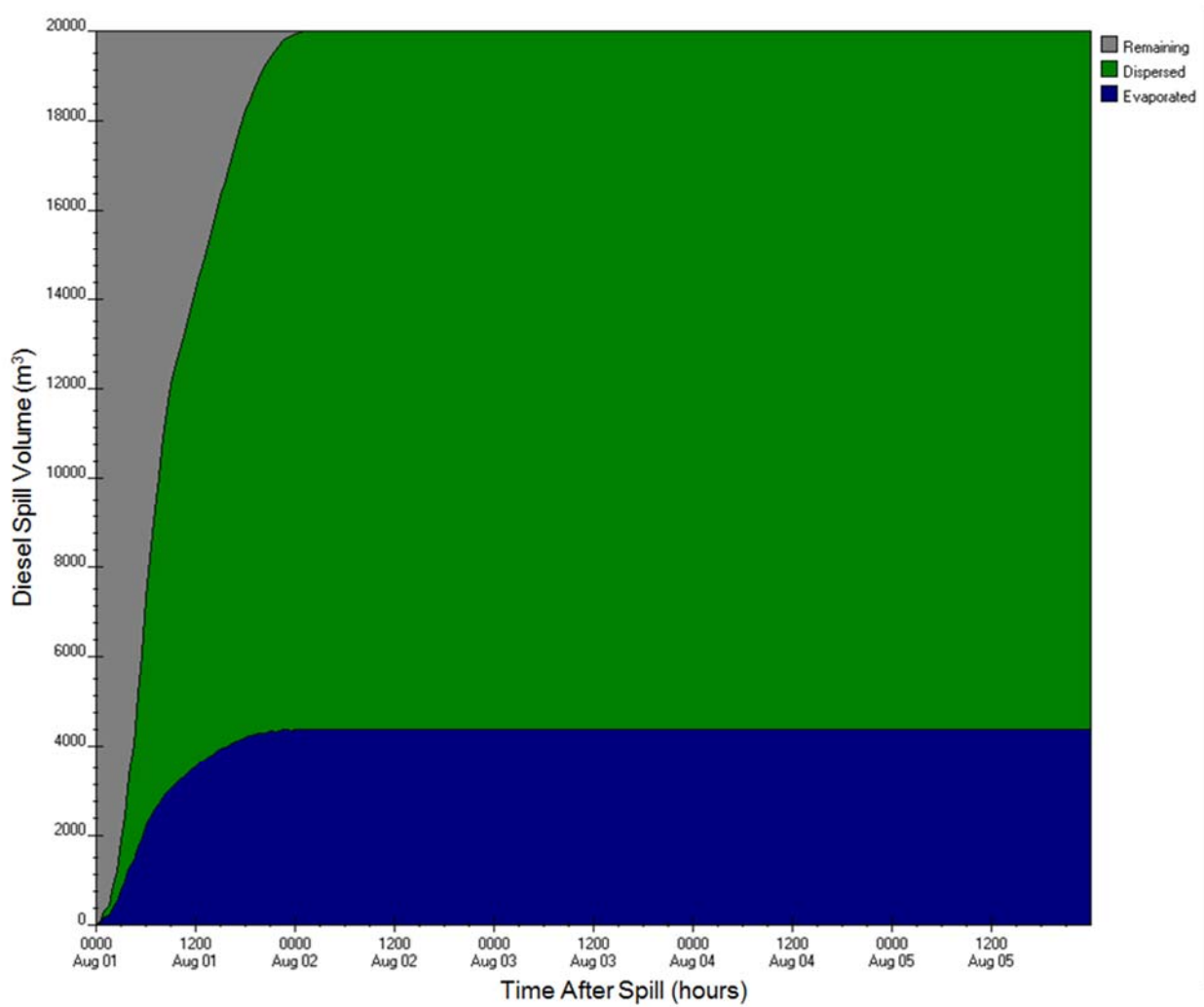
Figure E-A59: ADIOS2 diesel fuel budget output for Hudson Bay crossing station (5A) for 20,000 m 3 , 2-yr wind speed scenario
