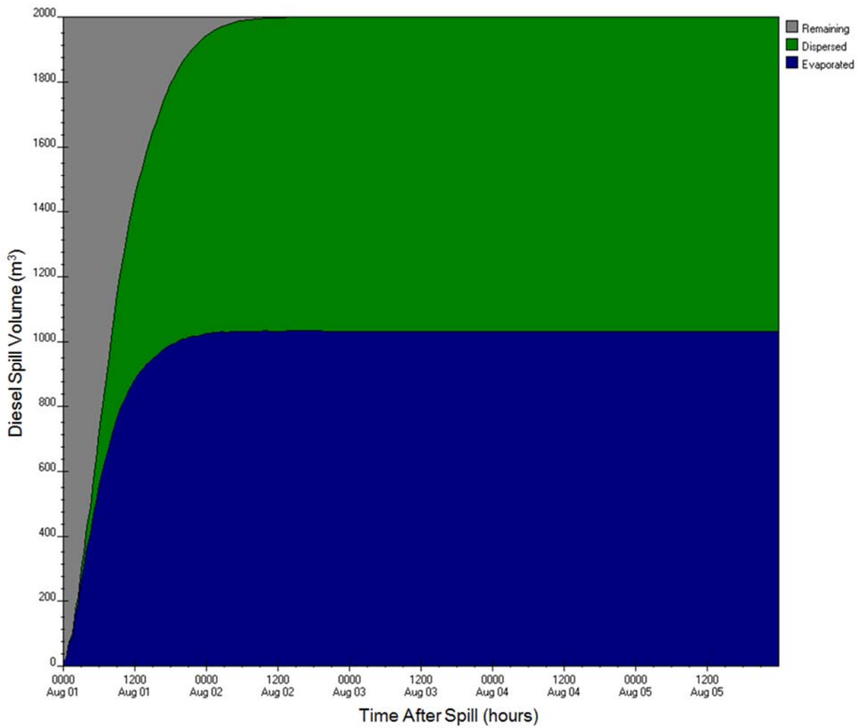
Figure E-A45: ADIOS2 diesel fuel budget output for Entrance to Melvin Bay station (3A) for 2,000 m 3 , 50-yr wind speed scenario
