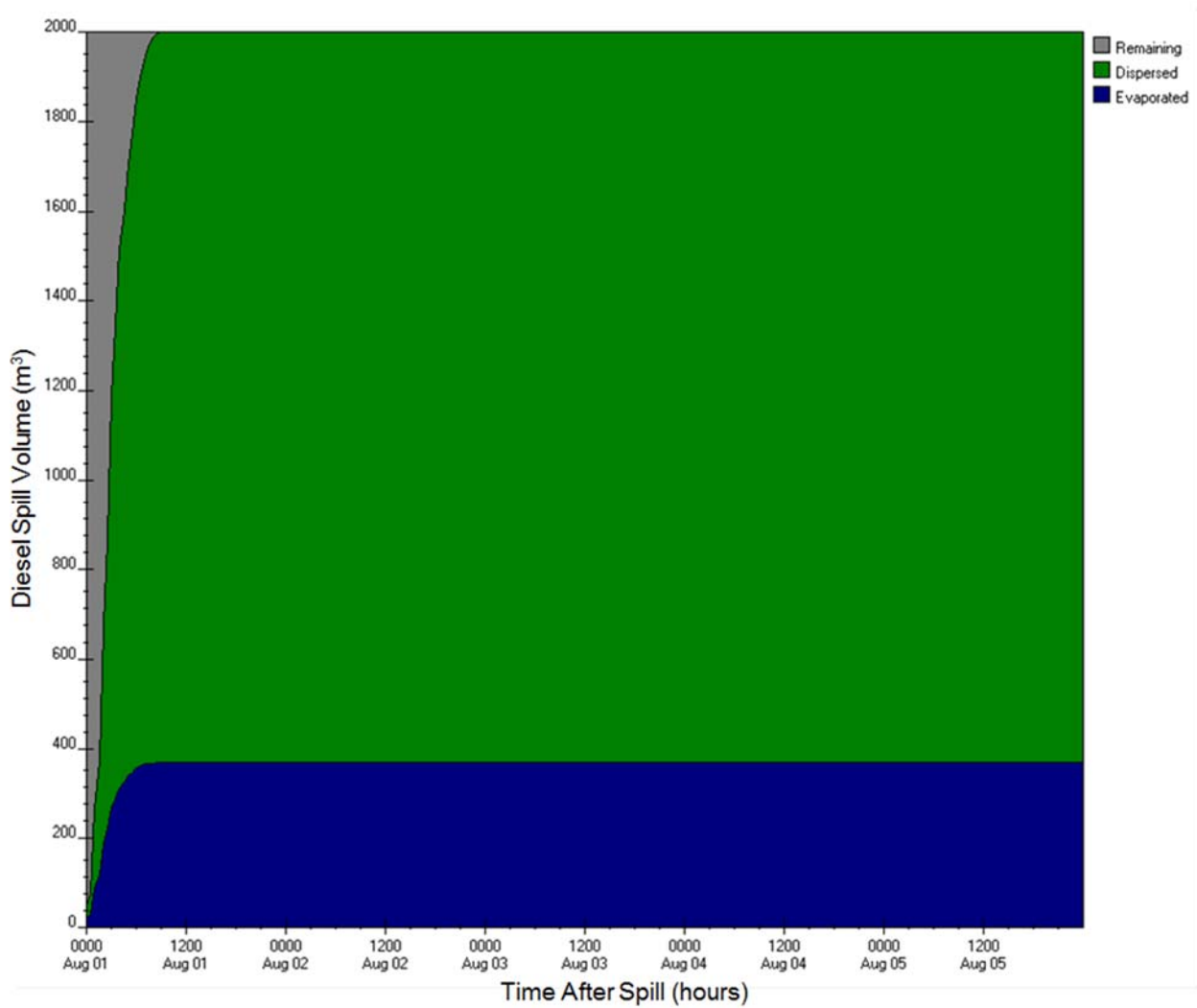
Figure E-A57: ADIOS2 diesel fuel budget output for Hudson Bay crossing station (5A) for 2,000 m 3 , 50-yr wind speed scenario
