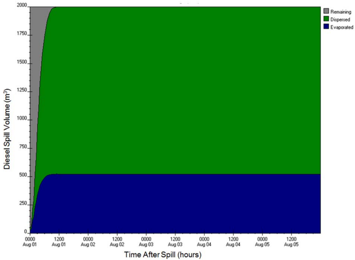
Figure E-A68: ADIOS2 diesel fuel budget output for Mid Hudson Strait station (7A) for 2,000 m 3 , 50-yr wind speed scenario
