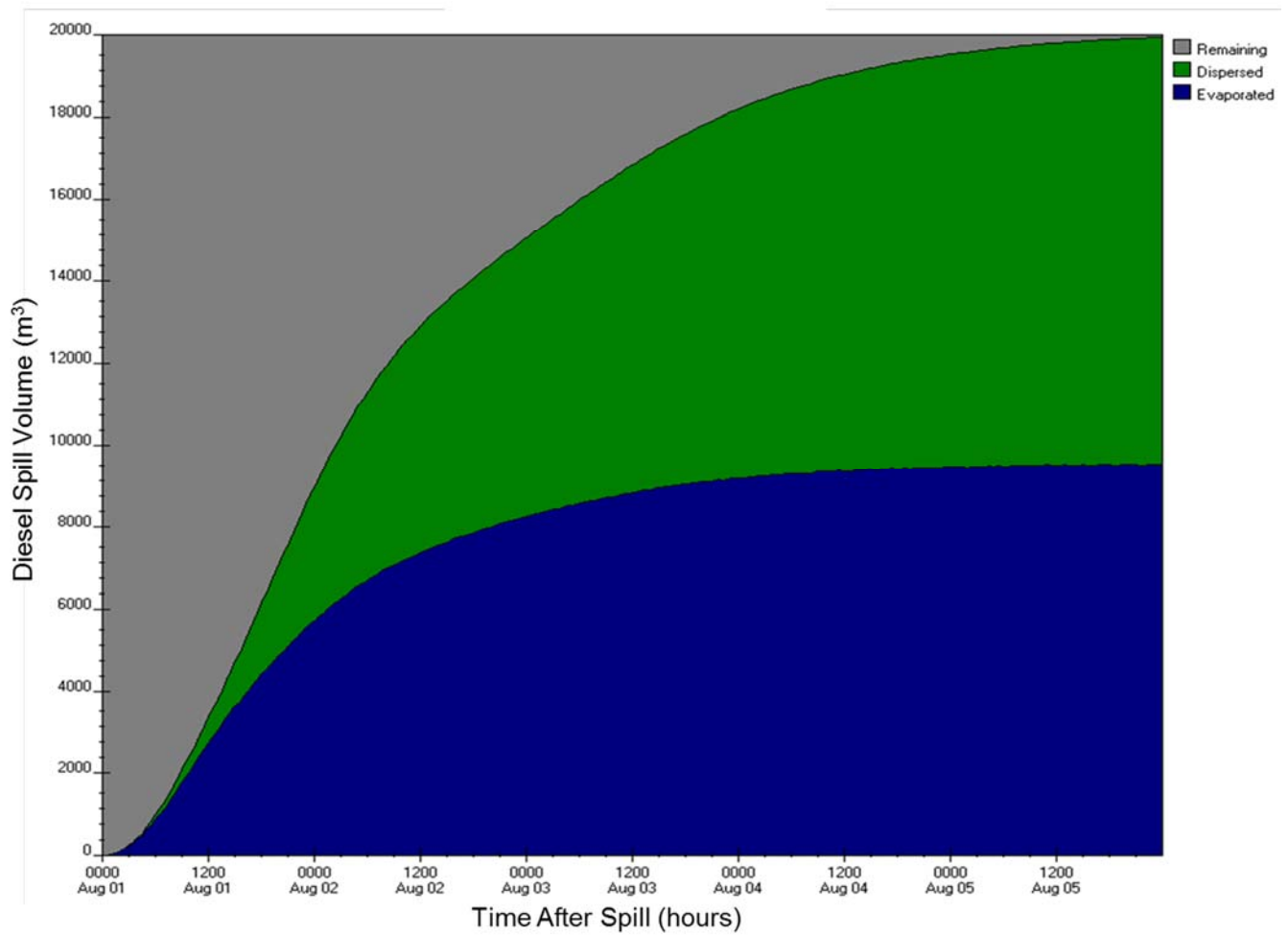
Figure E-A19: ADIOS2 diesel fuel budget output for Coats Island station (4) for 20,000 m 3 , mean wind speed scenario
