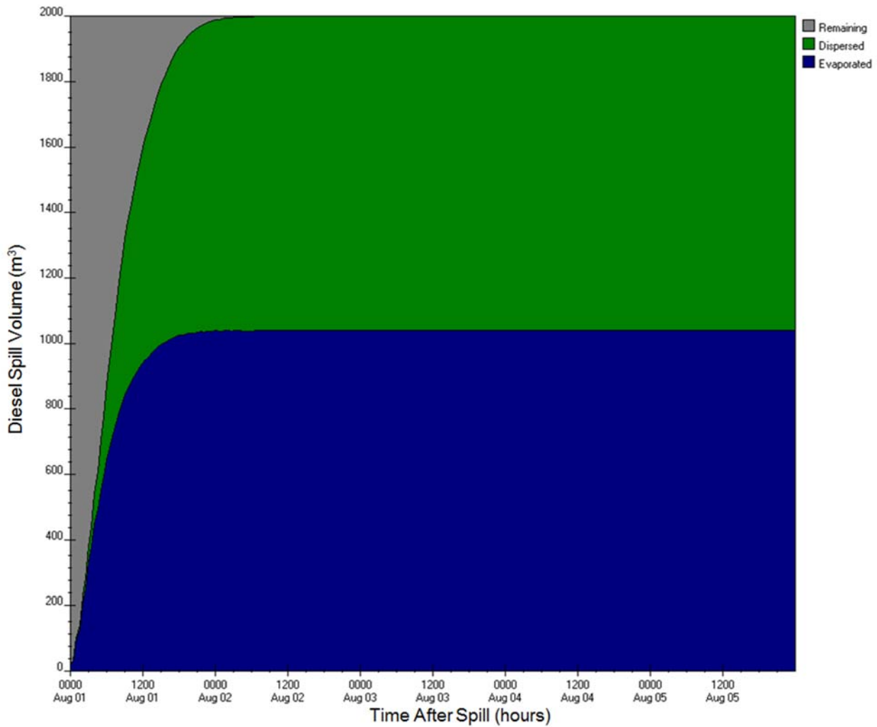
Figure E-A39: ADIOS2 diesel fuel budget output for West and East Melvin Bay stations (1A and 2A) for 2,000 m 3 , 50-yr wind speed scenario
