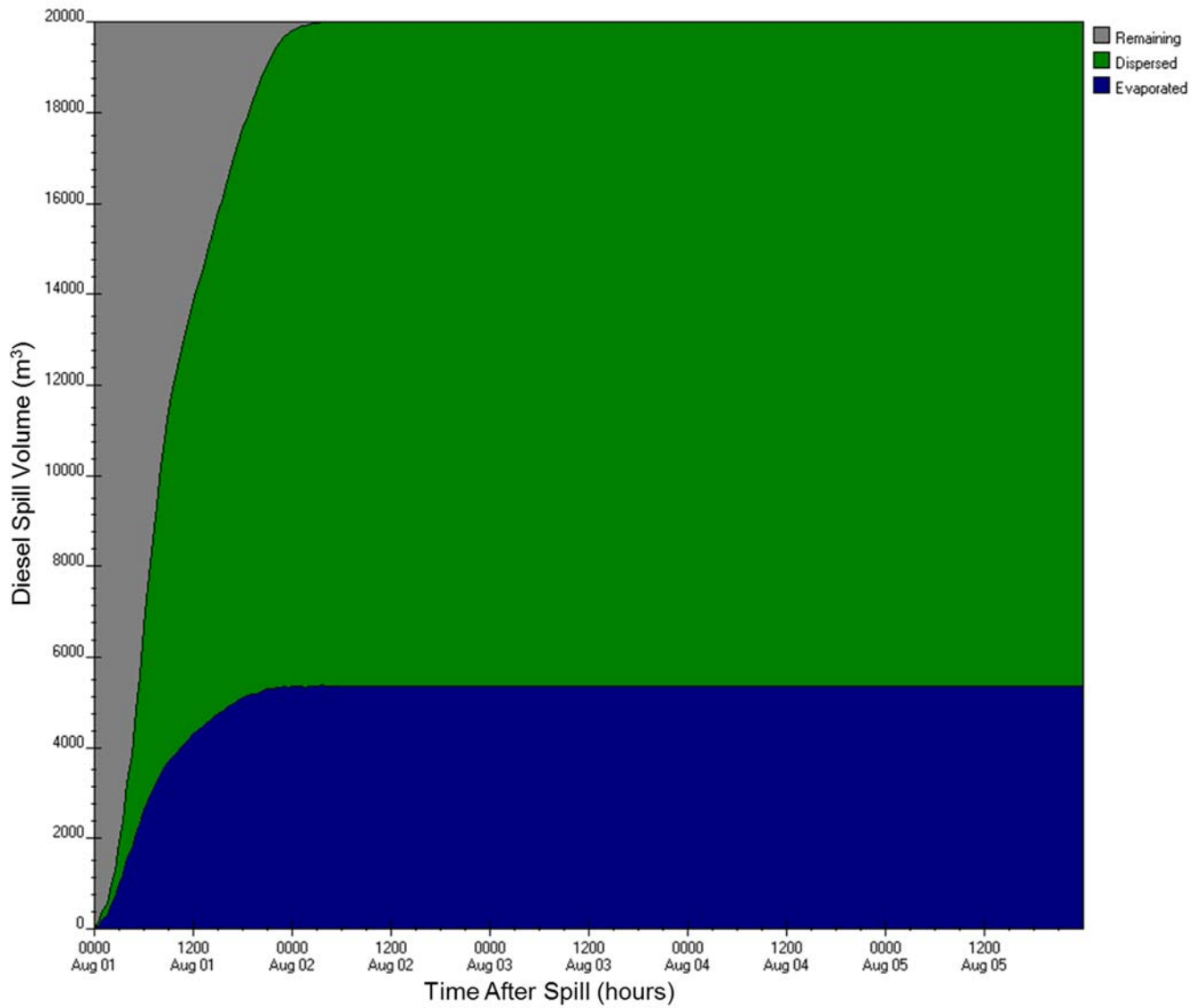
Figure E-A14: ADIOS2 diesel fuel budget output for Walrus Island station (3) for 20,000 m 3 , 2-yr wind speed scenario
