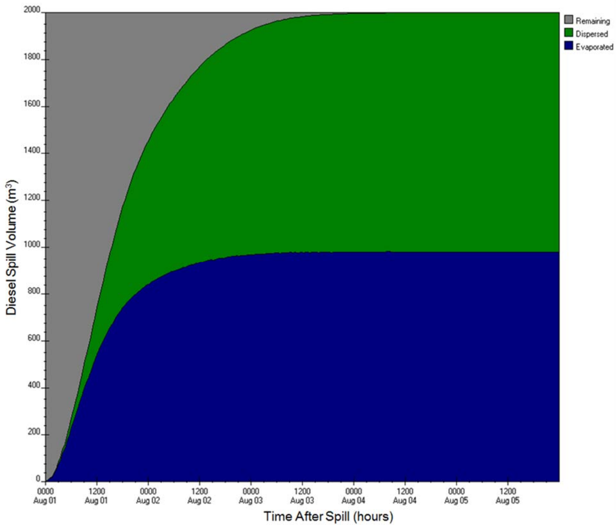
Figure E-A61: ADIOS2 diesel fuel budget output for Western Hudson Strait, Charles Island station (6A) for 2,000 m 3 , mean wind speed scenario
