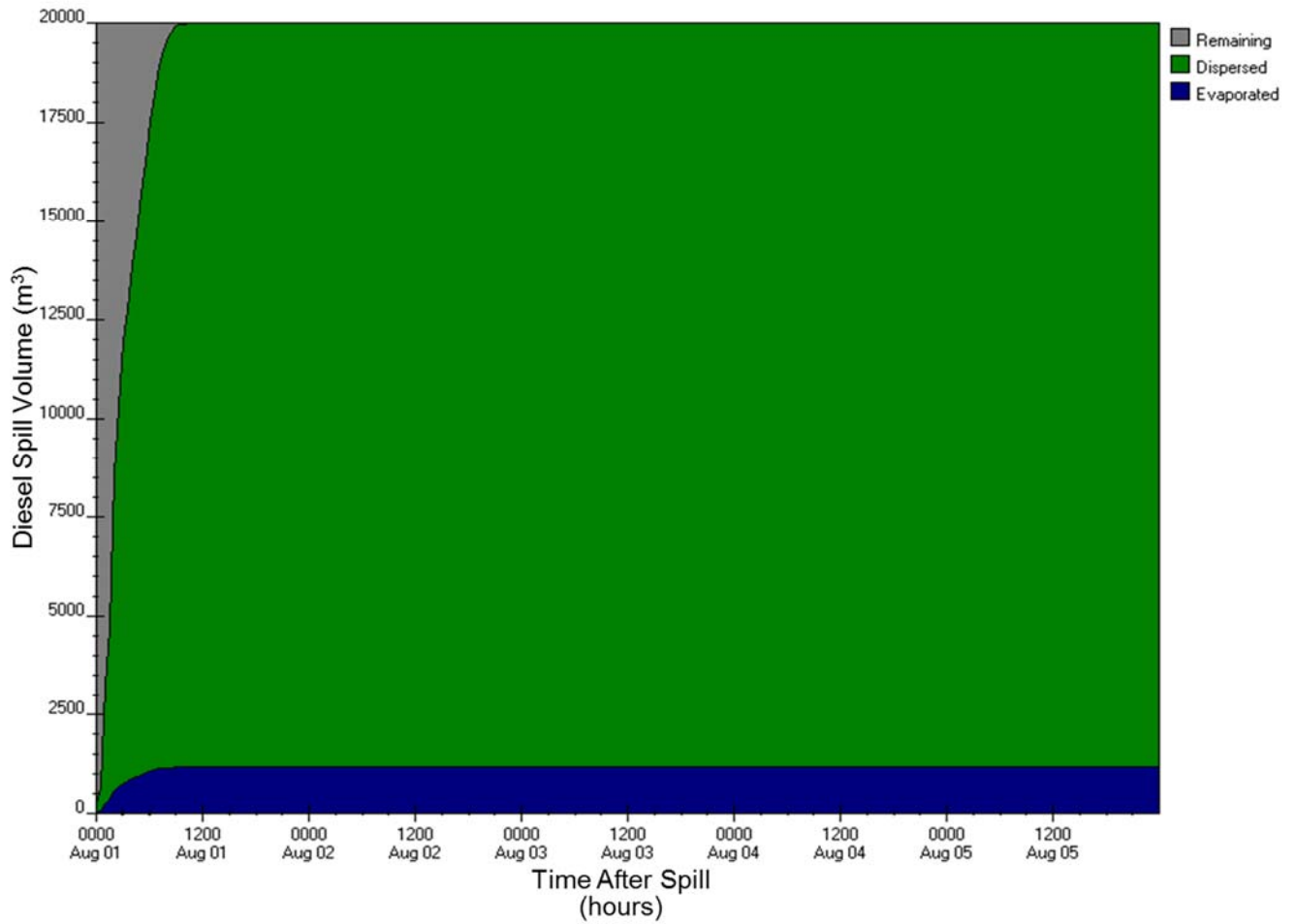
Figure E-A33: ADIOS2 diesel fuel budget output for Eastern Hudson Strait station (6) for 20,000 m³, 50-yr wind speed scenario
