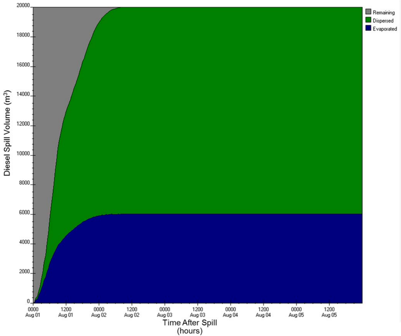
Figure E-A32: ADIOS2 diesel fuel budget output for Eastern Hudson Strait station (6) for 20,000 m 3 , 2-yr wind speed scenario
