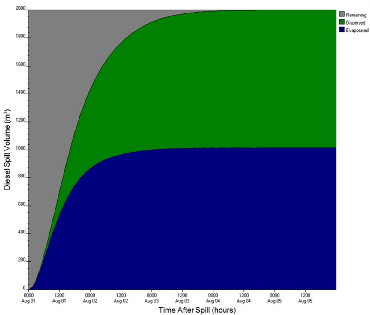
Figure E-A67: ADIOS2 diesel fuel budget output for Mid Hudson Strait station (7A) for 2,000 m 3 , mean wind speed scenario
