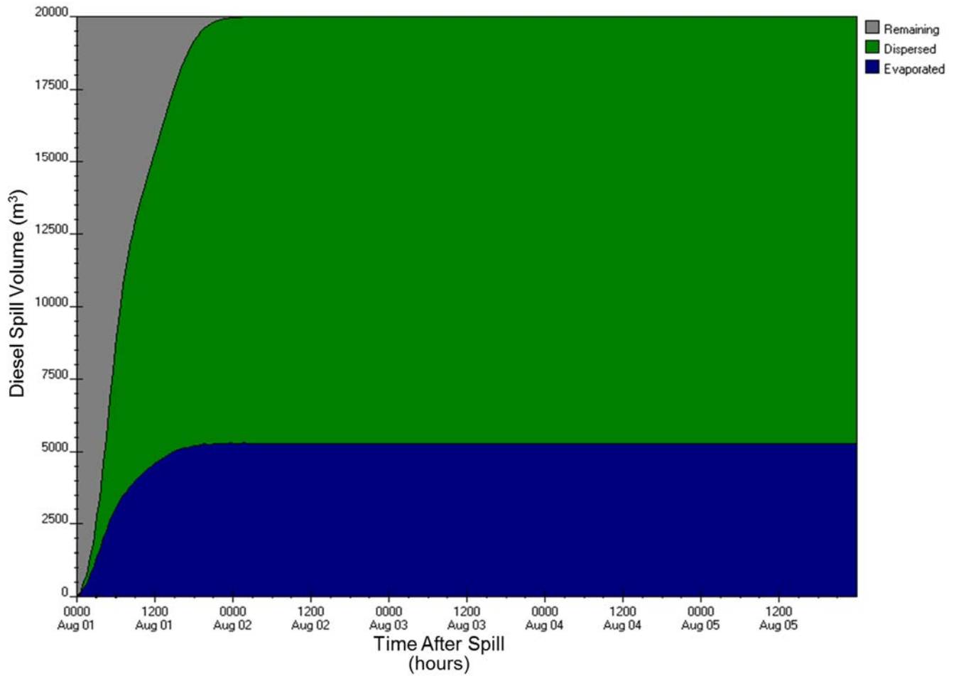
Figure E-A27: ADIOS2 diesel fuel budget output for Ungava Peninsula station (5) for 20,000 m 3 , 50-yr wind speed scenario
