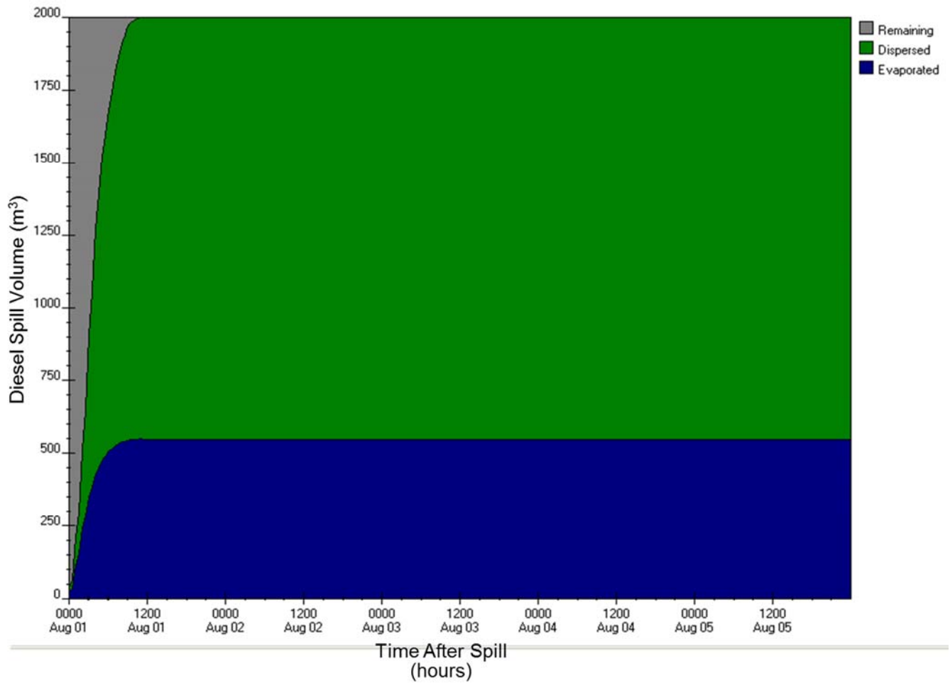
Figure E-A24: ADIOS2 diesel fuel budget output for Ungava Peninsula station (5) for 2,000 m 3 , 50-yr wind speed scenario
