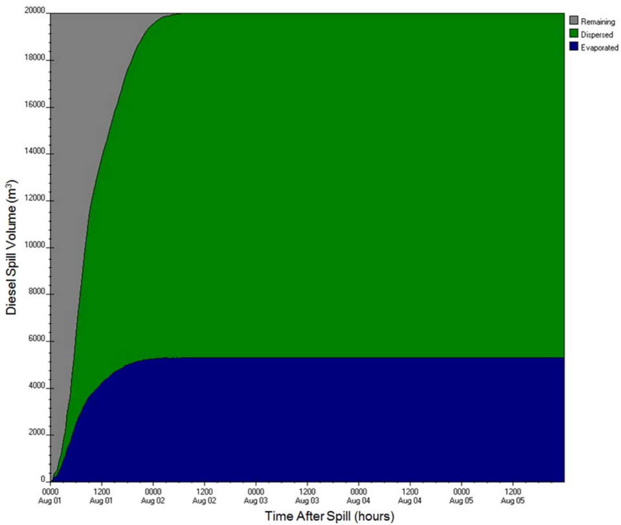
Figure E-A70: ADIOS2 diesel fuel budget output for Mid Hudson Strait station (7A) for 20,000 m 3 , 2-yr wind speed scenario
