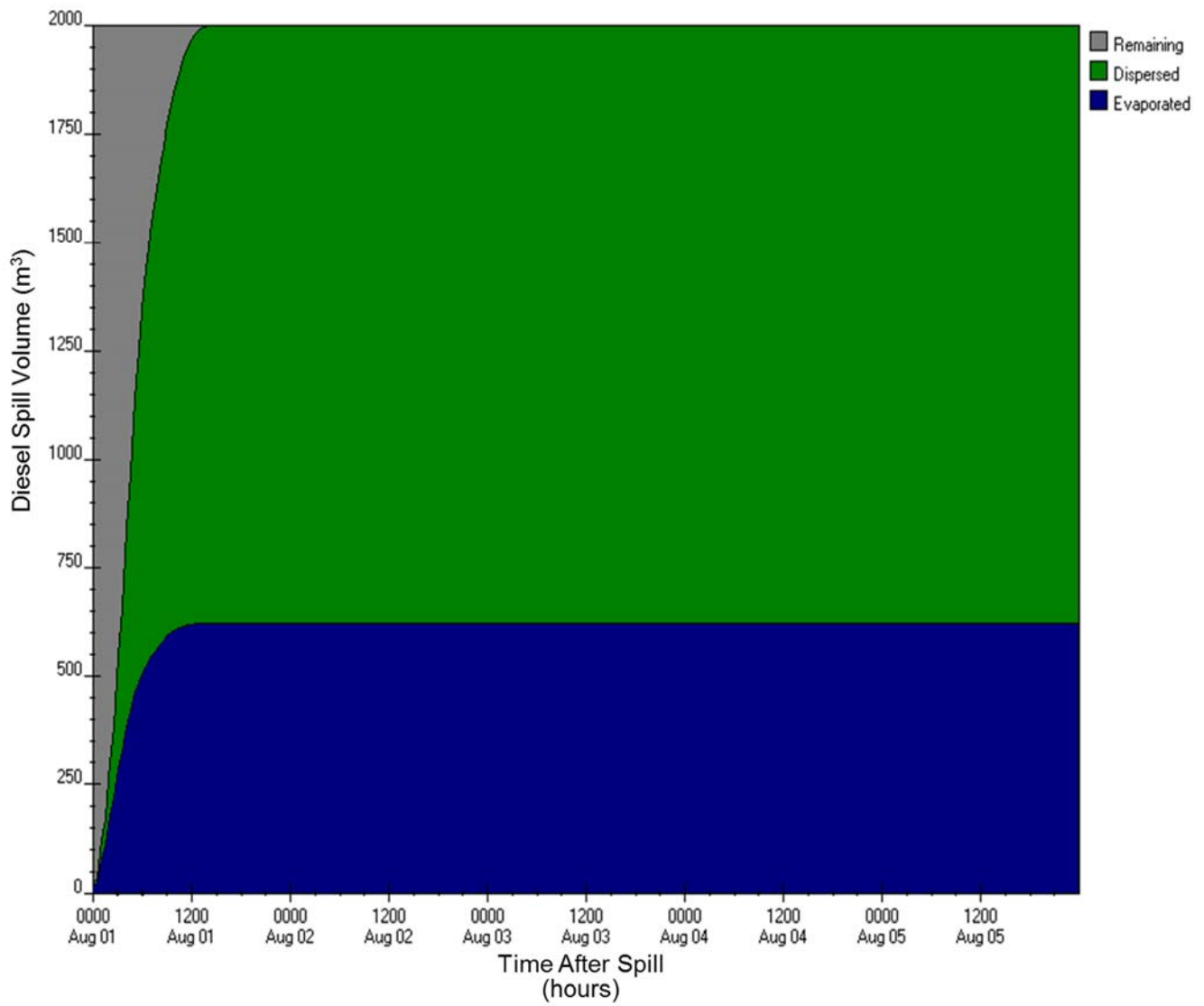
Figure E-A29: ADIOS2 diesel fuel budget output for Eastern Hudson Strait station (6) for 2,000 m 3 , 2-yr wind speed scenario
