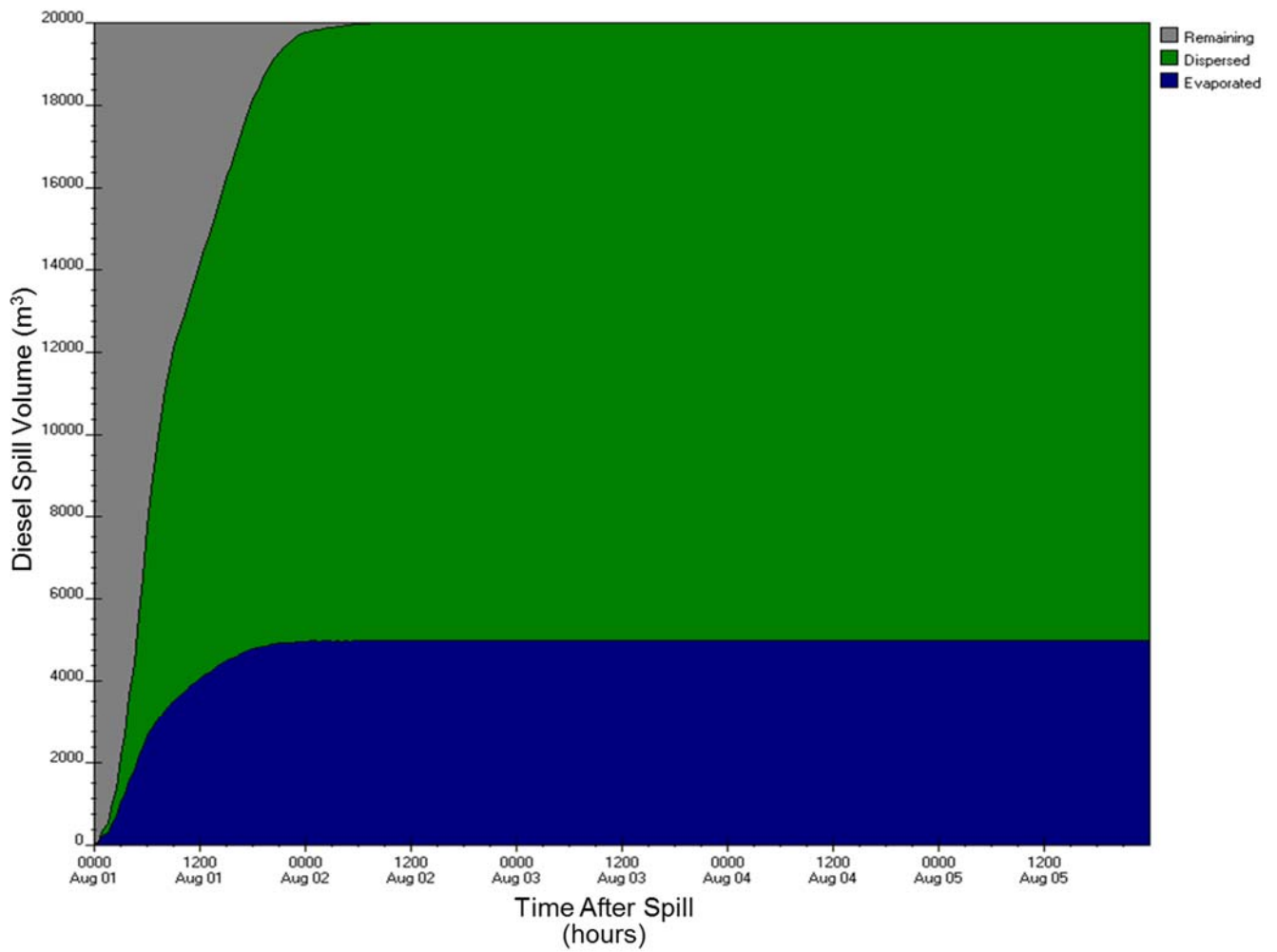
Figure E-A20: ADIOS2 diesel fuel budget output for Coats Island station (4) for 20,000 m 3 , 2-yr wind speed scenario
