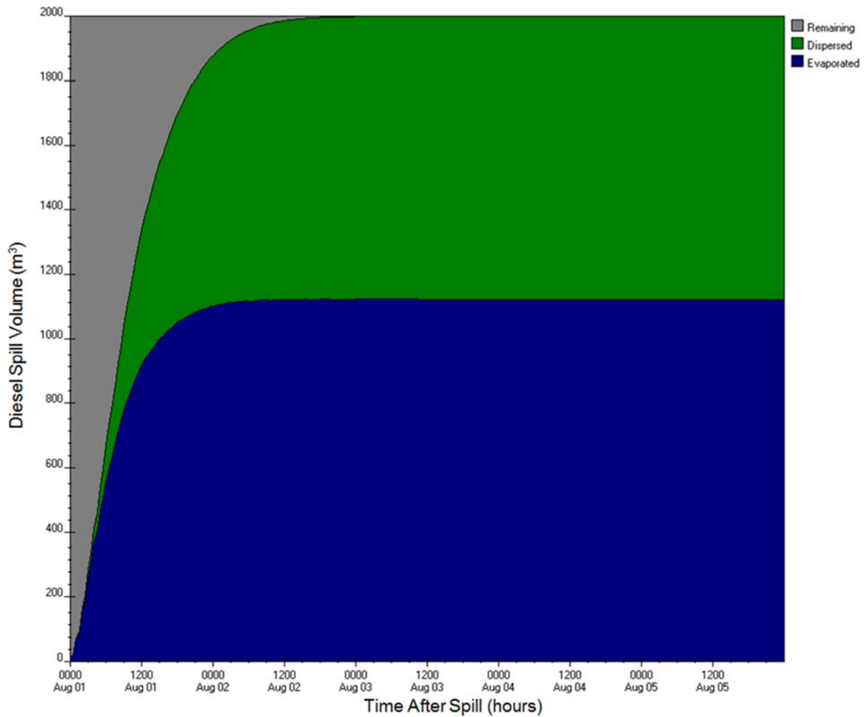
Figure E-A38: ADIOS2 diesel fuel budget output for West and East Melvin Bay stations (1A and 2A) for 2,000 m 3 , 2-yr wind speed scenario
