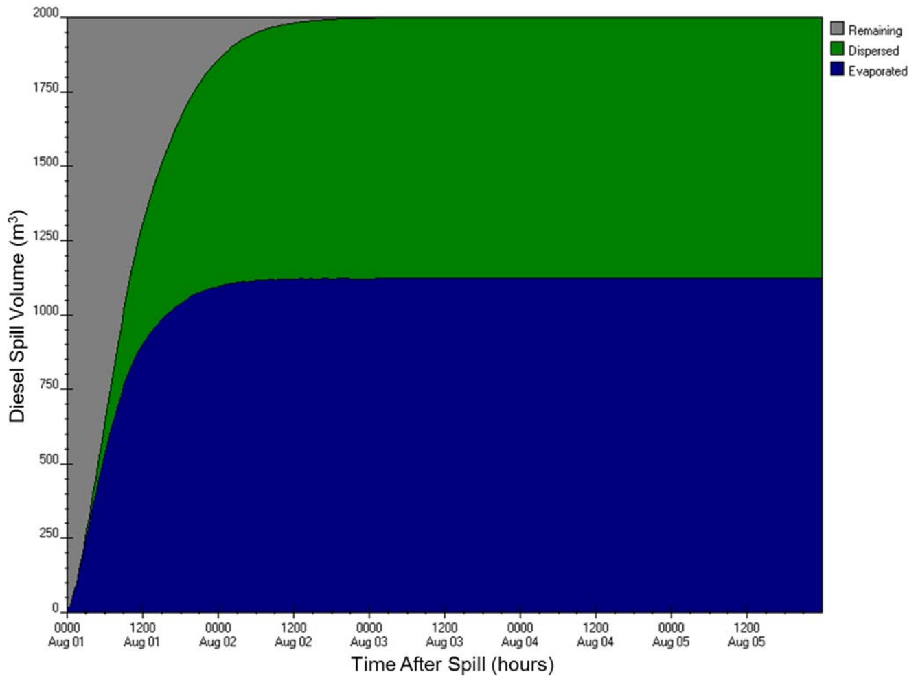
Figure E-A5: ADIOS2 diesel fuel budget output for two fuel transfer stations (1 and 2) near Melvin Bay for 2,000 m 3 , 2-yr wind speed scenario
