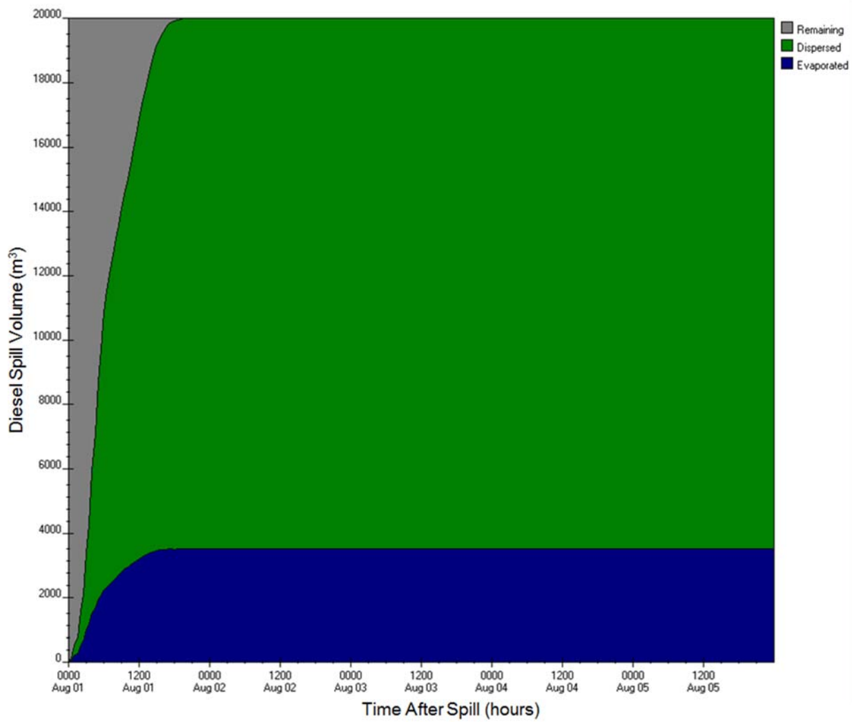
Figure E-A65: ADIOS2 diesel fuel budget output for Western Hudson Strait, Charles Island station (6A) for 20,000 m 3 , 2-yr wind speed scenario
