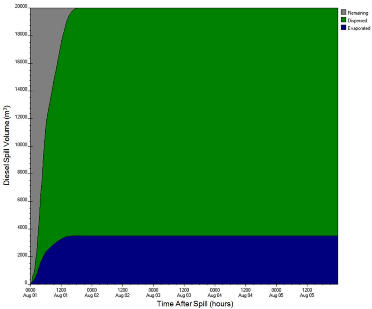
Figure E-A60: ADIOS2 diesel fuel budget output for Hudson Bay crossing station (5A) for 20,000 m 3 , 50-yr wind speed scenario
