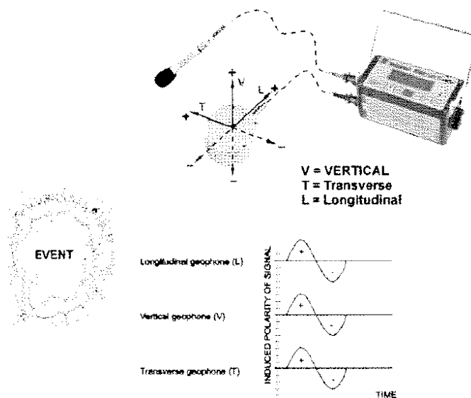
Figure 2. Sensor Orientation
