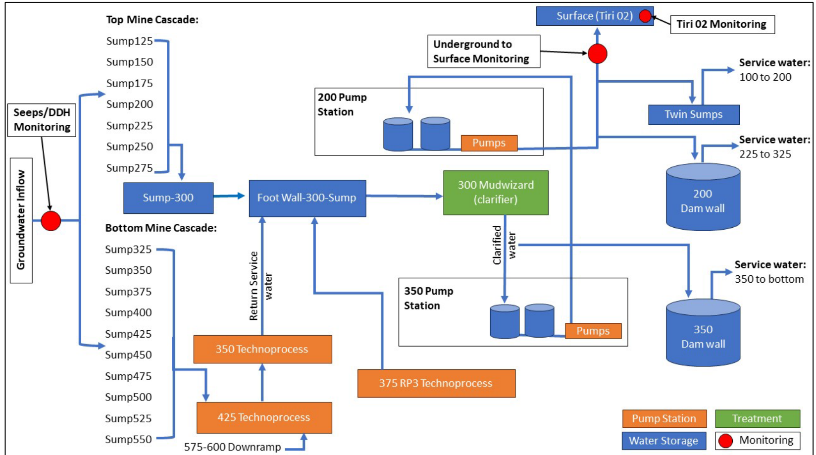
Figure 1: Simplified underground water management flow sheet diagram.
