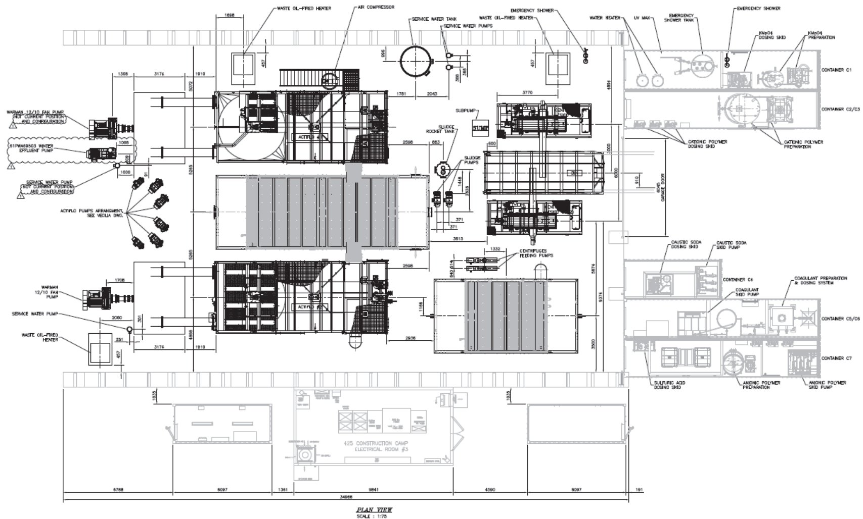
Figure 2 – General Arrangement of ASWTP
