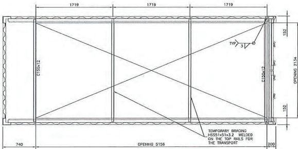
PLAN VIEW - FLOOR SCALE: 1:25
