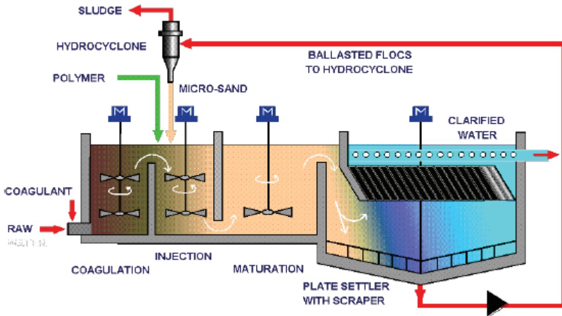
Figure 5 – Actiflo® Process
